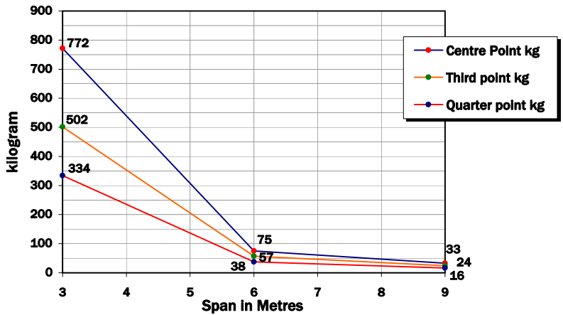
300mm Flat Truss "MID POINT RESTRAINT" Centre/Third/Quarter point loads.
