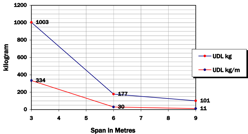
300mm Flat Truss "MID POINT RESTRAINT" UDL (uniform distributed load)
